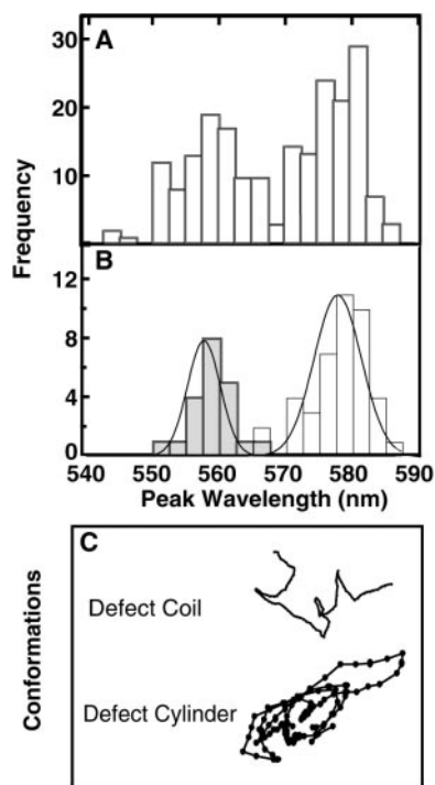
Fig. 2. (A) Distribution of the peak wavelength ( \lambda_{\text{max}} ) of single-molecule fluorescent spectra of MEH-PPV found by simply finding the maxima in spectra analogous to Fig. 1B. Histogram was constructed from data of several different samples using the same sample preparation procedure. (B) Two histograms plotted in different shades, which represent data taken from two different areas in the same sample film. (C) "Snapshot" of the defect-coil conformation and defect-cylinder conformation of a single polymer chain (9).
