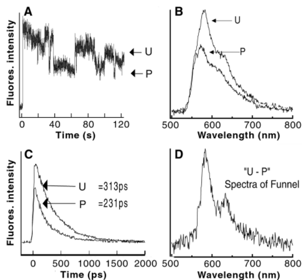
Fig. 4. (A) The time-dependent fluorescence intensity of a single MEH-PPV molecule undergoing intensity fluctuations due to quenchers induced by excitation at 470 to 480 nm with a frequency-doubled Ti:sapphire laser (repetition rate = 76 MHz). Similar transients are observed for cw excitation (488 nm) as in Fig. 3. (B) “Sorted” single-molecule fluorescent spectra of the U and P states. (C) Sorted single-molecule time-resolved kinetic traces of the U and P states, recorded by the time-correlated single-photon counting technique with a microchannel plate detector. Lifetimes ( \tau ) were obtained for each trace by single-exponential fitting. (D) The difference (U – P) between the U and P emission spectra.
